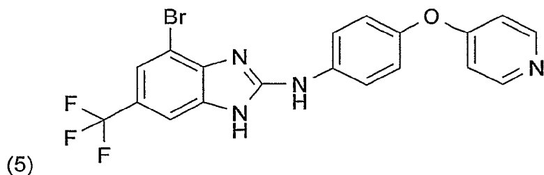
(4-Brom-6-trifluormethyl-1H-benzimidazol-2-yl)-[4-(pyridin-4-yloxy)-phenyl]-amin
